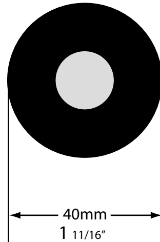
Part No. E-20 Fits E-100 Style Headphones
